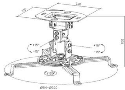
Dimensions (mm)
